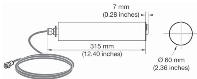
SOLITAX sc Immersion Probe
